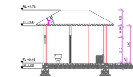
SECTION 3-S3
