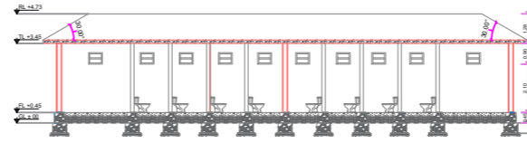
SECTION 1-S1
