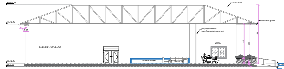
SECTION 2-S2
