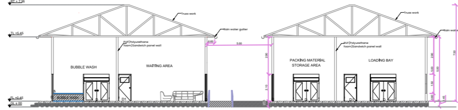
SECTION 1-S1
