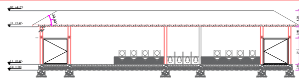
SECTION 2-S2
